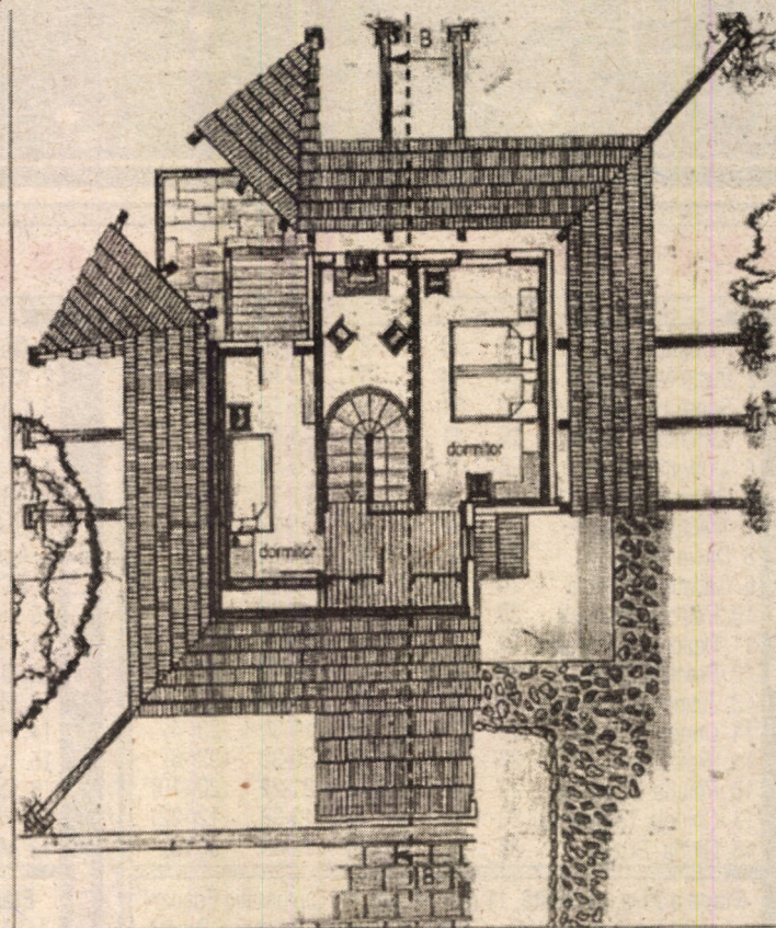
Plan mansardă
