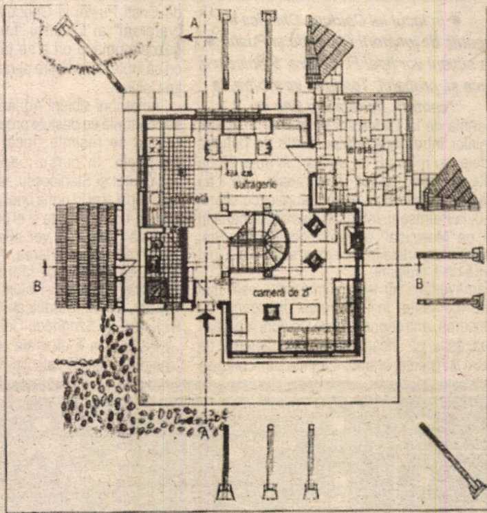
Plan parter
